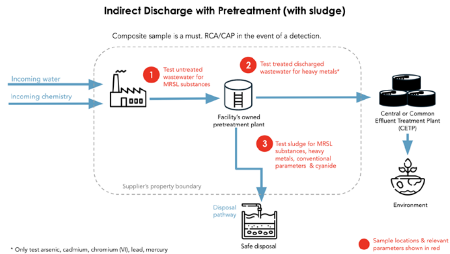
Figure 1b: Schematic illustration of the sample locations for an indirect discharge, with pretreatment (with sludge) supplier. Sampling locations: untreated wastewater, discharged wastewater, sludge
